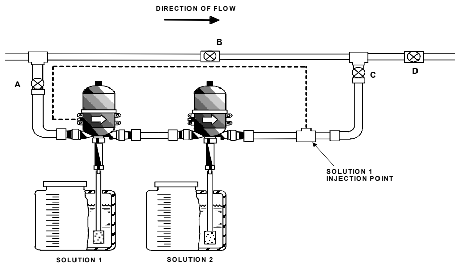
DUAL INSTALLATION WITH REMOTE INJECTION
